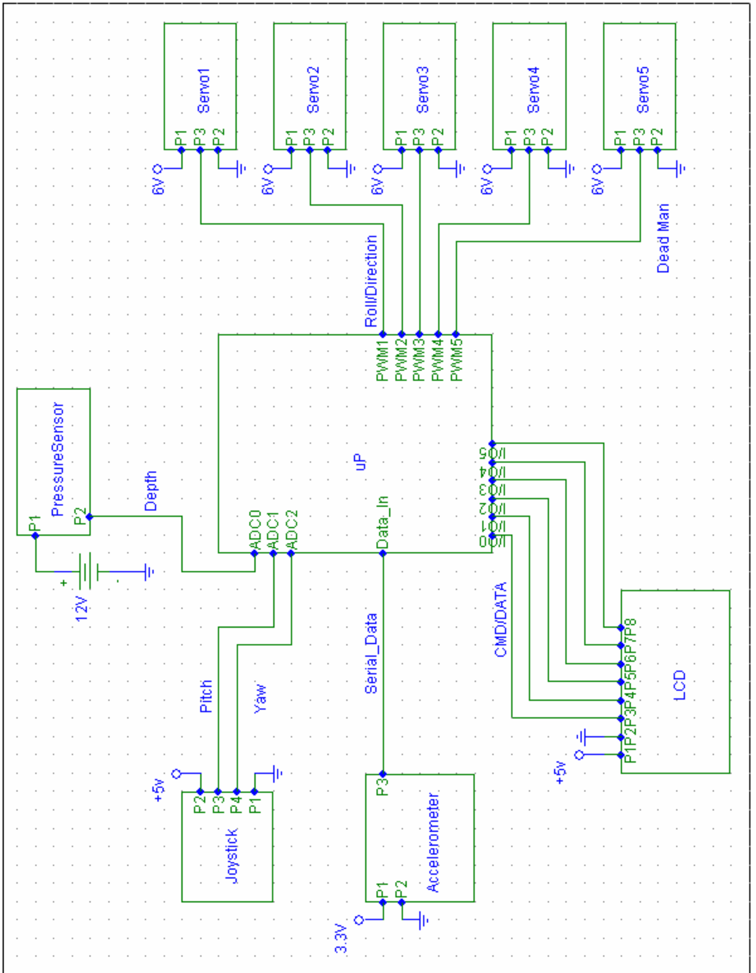
Charles Shupard – HPS Controls Block Diagram
